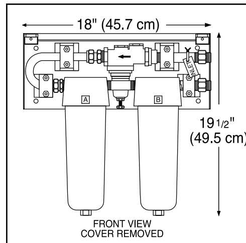
PREFILTER ASSEMBLY
